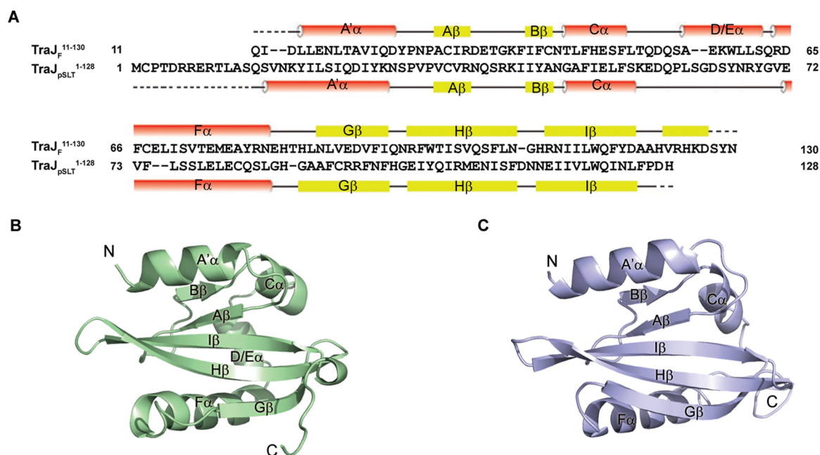
Figure 1. Overall structures of TraJ F 11-130 and TraJ pSLT 1-128 . (A) Alignment of amino acid sequences of TraJ F 11-130 and TraJ pSLT 1-128 . Secondary structure elements of TraJ F 11-130 and TraJ pSLT 1-128 are shown above and below the corresponding sequences, respectively. Dotted lines indicate residues not modeled in the crystal structures because of a lack of electron density. (B) Crystal structure of a TraJ F 11-130 monomer. Secondary structural elements as well as the N- and C-termini are labeled. (C) Crystal structure of a TraJ pSLT 1-128 monomer.
