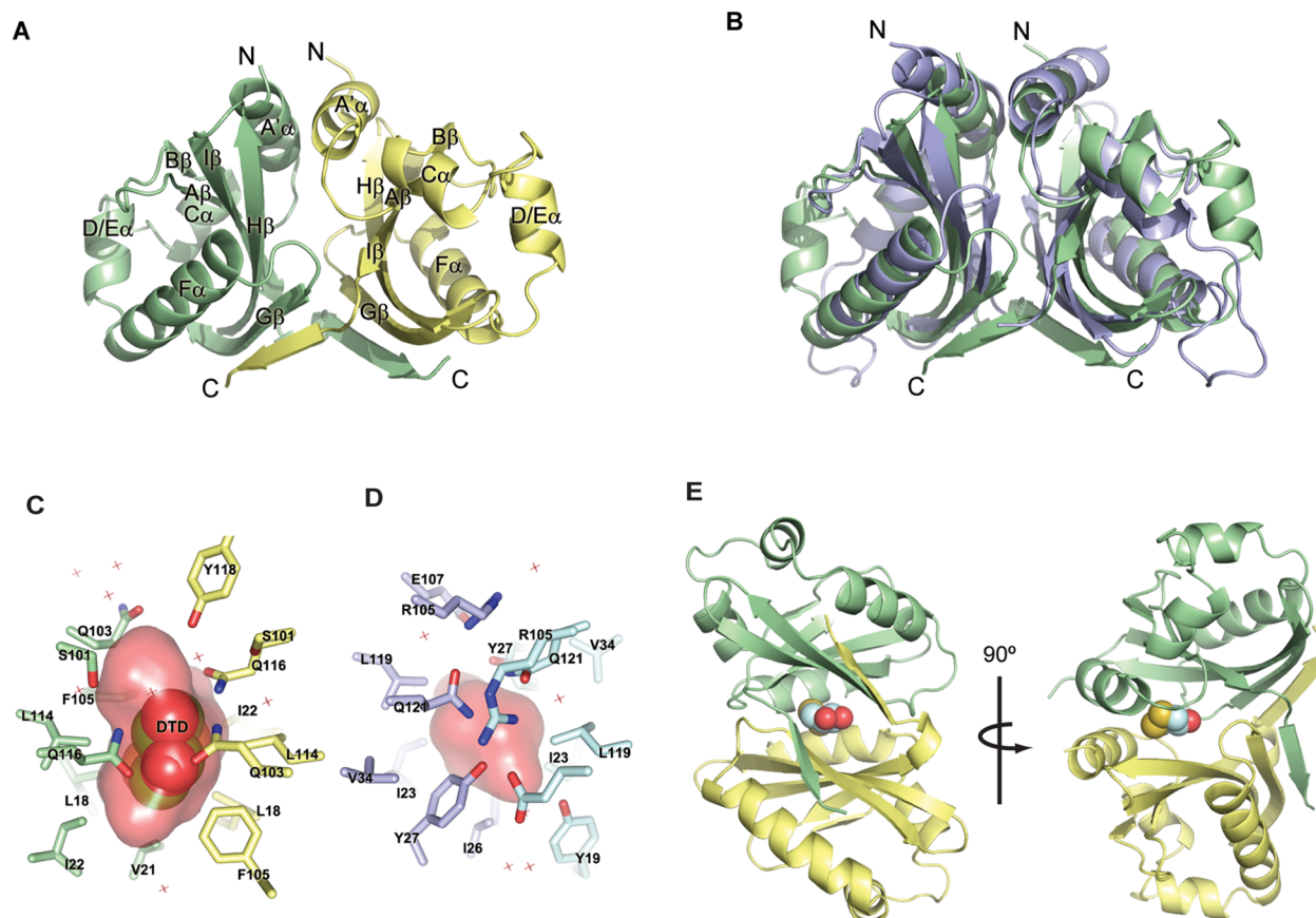
Figure 2. Homodimerization of TraJ F 11–130 and TraJ pSLT 1–128 . The two protomers of each dimer are colored differently. (A) Crystal structure of a TraJ F 11–130 dimer. (B) Superposition of the TraJ F 11–130 (green) and TraJ pSLT 1–128 (blue) dimers. (C) TraJ F 11–130 residues surrounding DTD (shown as spheres) at the dimeric interface. The surface of the internal pocket is colored red. (D) Residues surrounding a small cavity at the dimeric interface of TraJ pSLT 1–128 . (E) Position of the DTD (spheres) pocket in the overall structure of a TraJ F 11–130 dimer.
